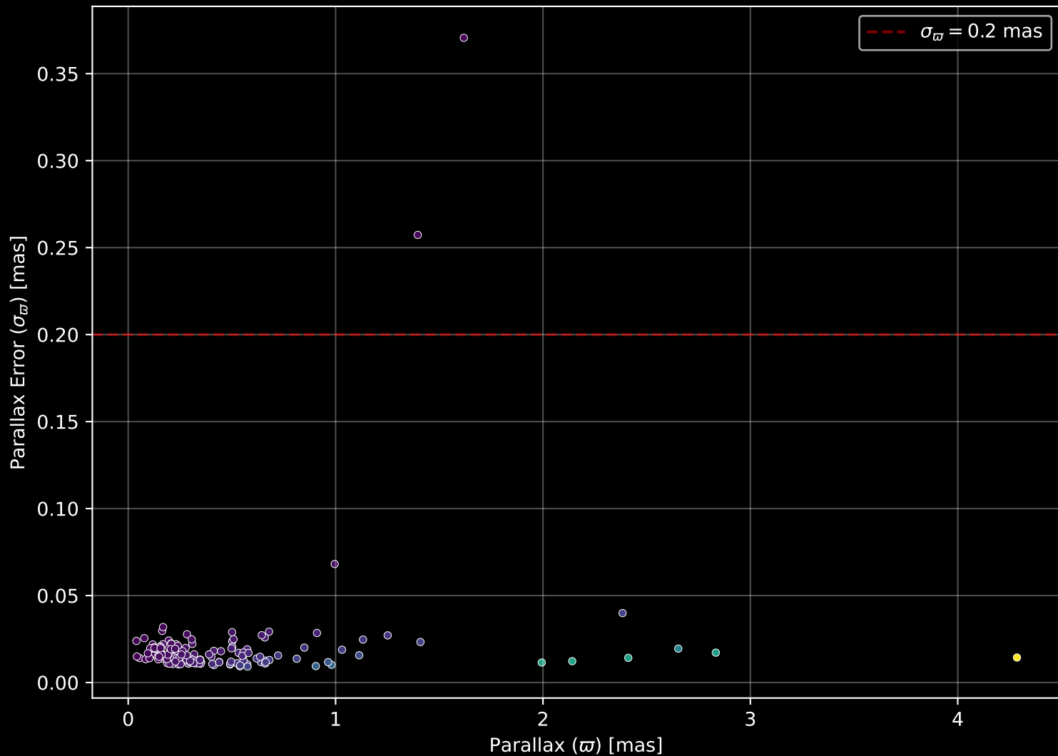
APOGEE DR17 Field: [101-04] Parallax Quality (n= 158)
