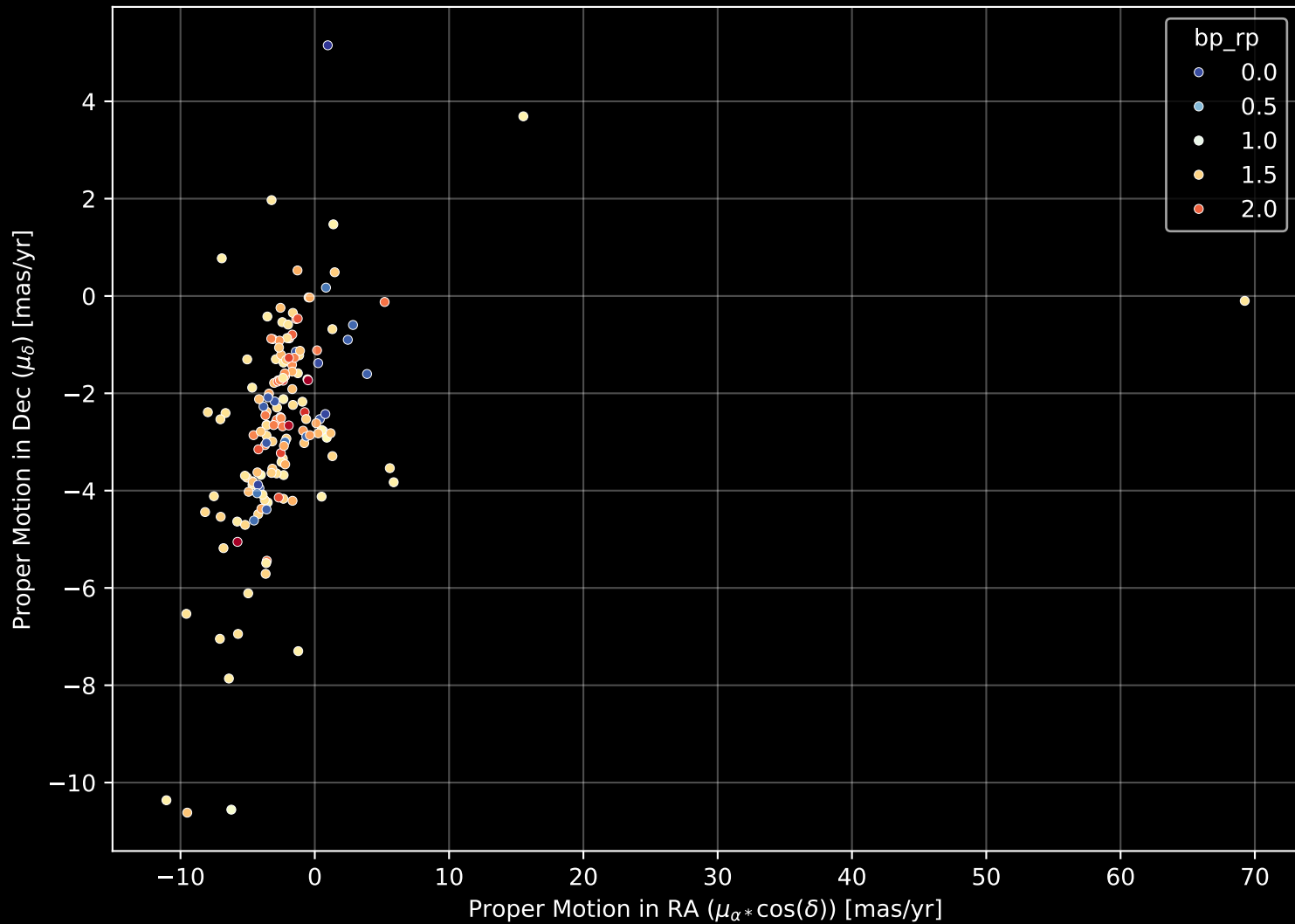
APOGEE DR17 Field: [101-04] Proper Motion Diagram (n= 158)
