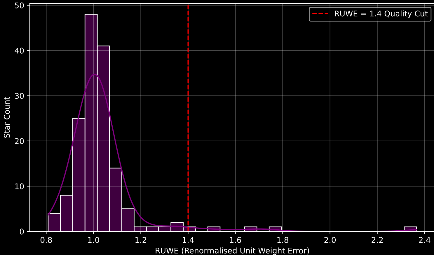
GAPOGEE DR17 Field [101-04] RUWE Distribution (n= 155)
