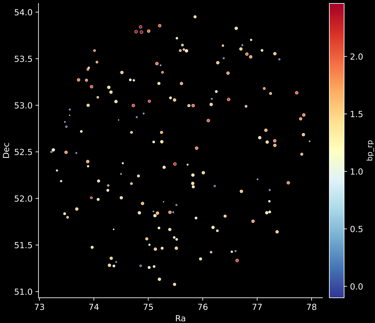
APOGEE DR17 Field: [101-04] Stars: 158
