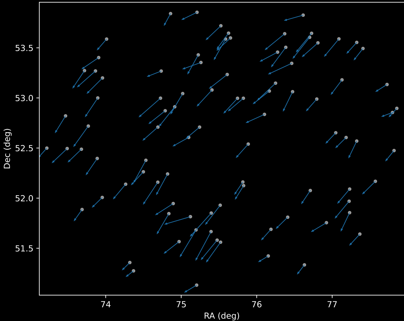
APOGEE DR17 Cluster 0 Proper Motion Vectors (n=90)
