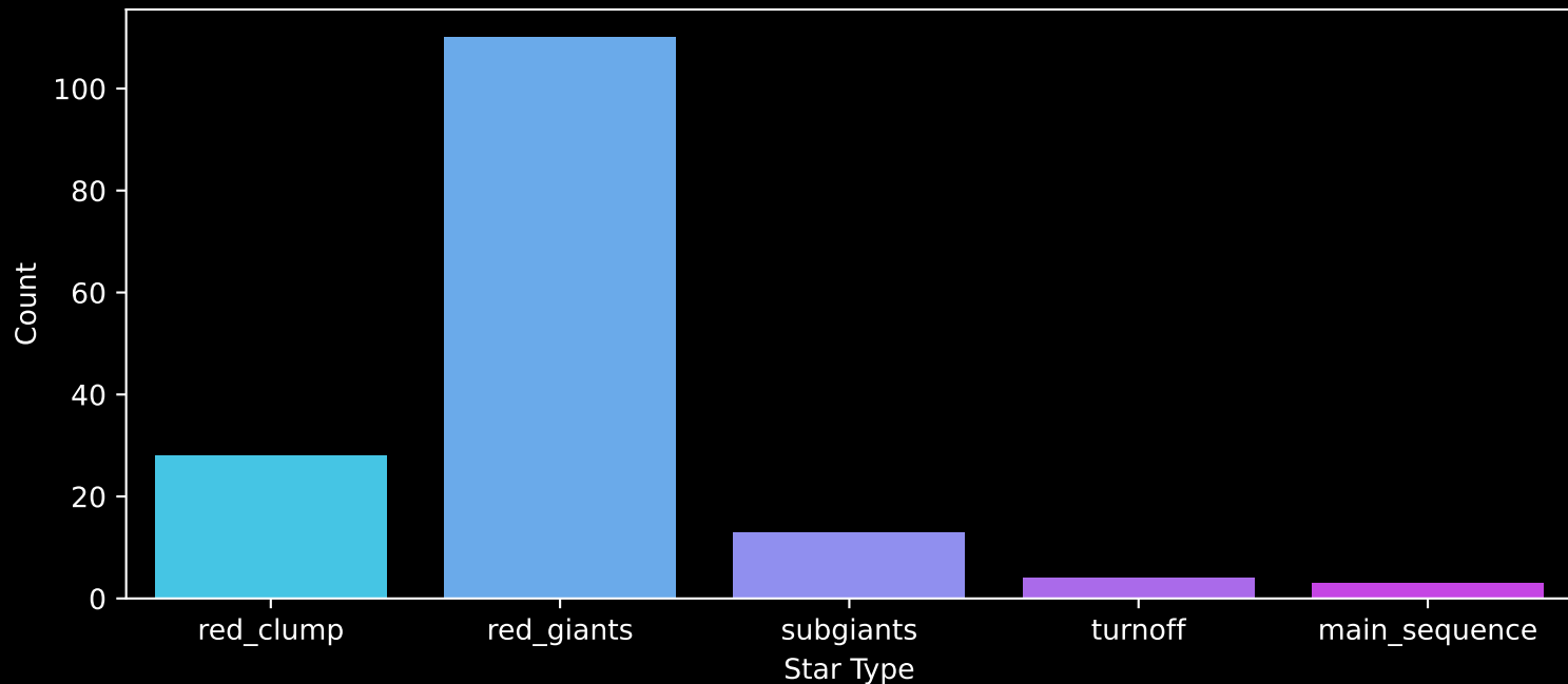
APOGEE DR17 Field: [101-04] Count plot of Star Type
