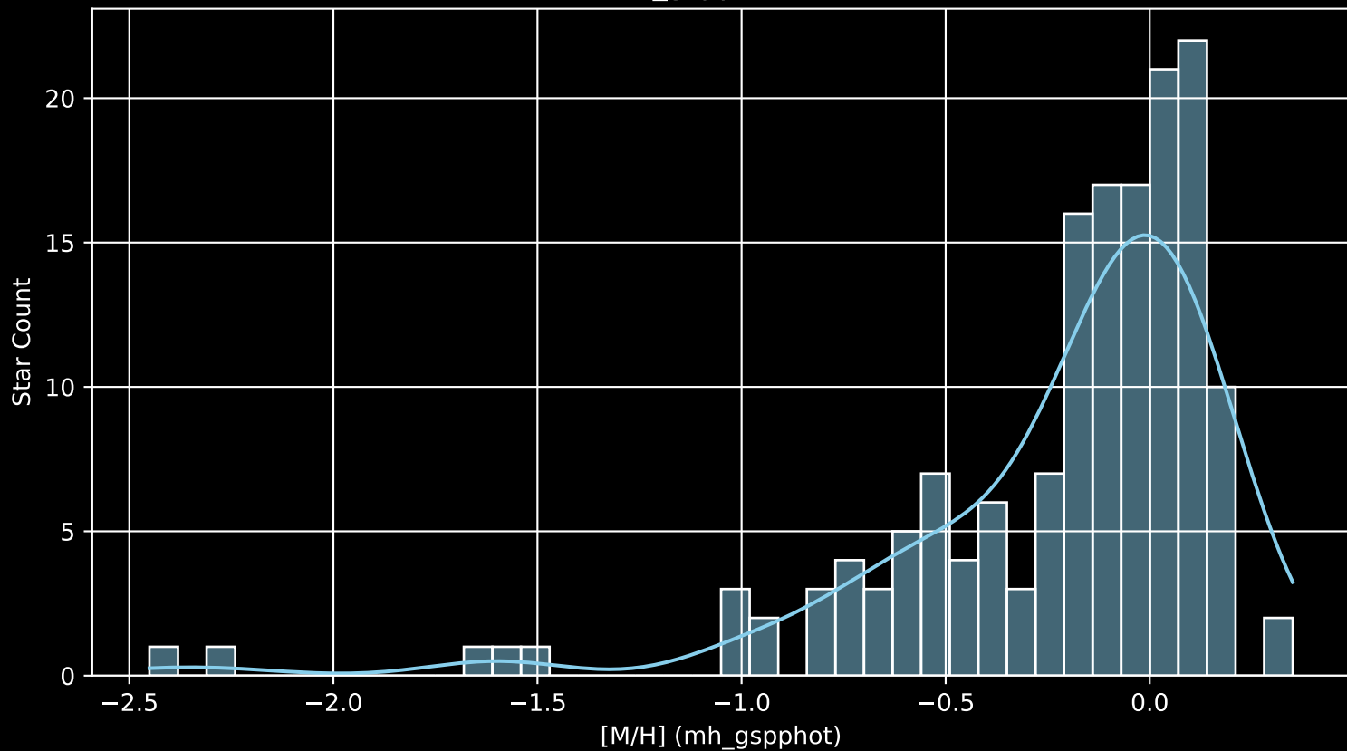
APOGEE DR17 Field: [101-04 [M/H] (mh_gspphot) (n= 157)
